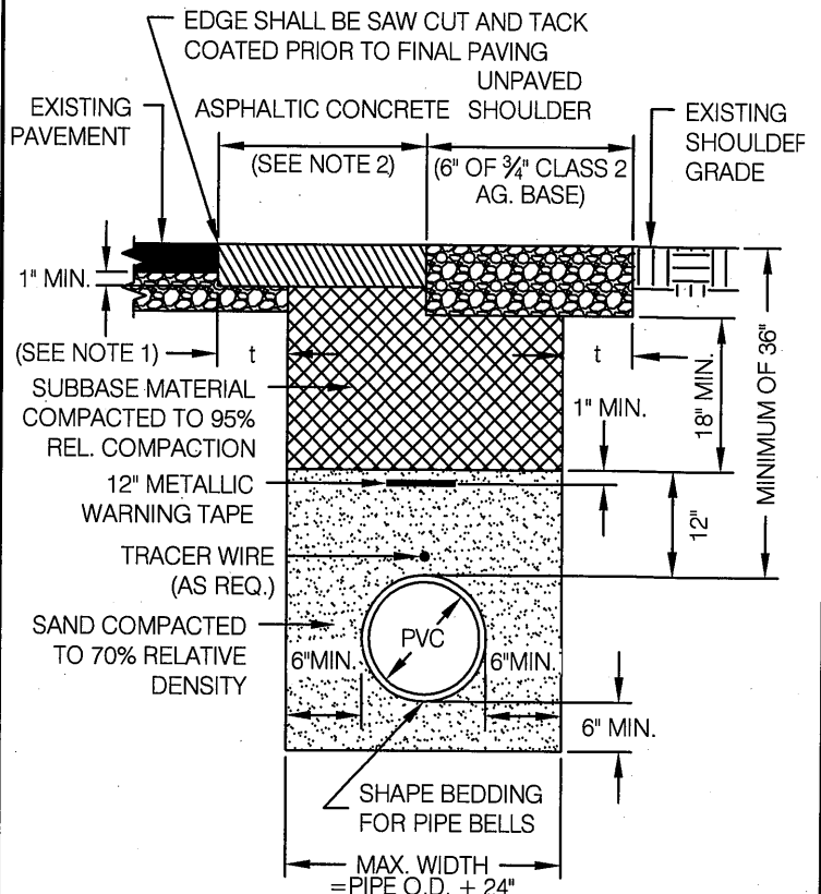
TRENCH IN EXISTING PAVED PORTIONS AND/OR UNPAVED SHOULDERS
