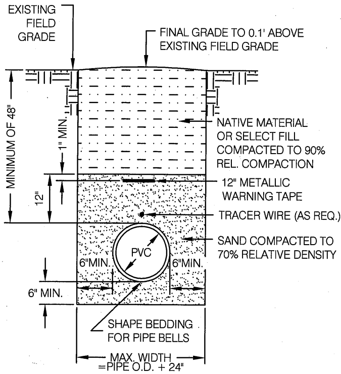
TRENCH IN OPEN AREAS
