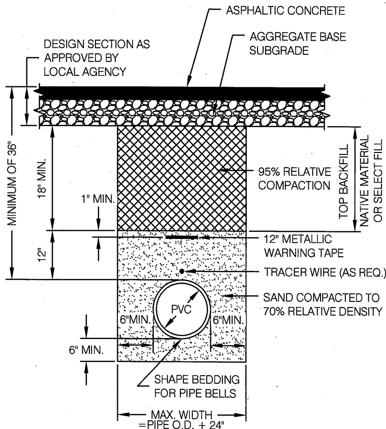
TRENCH IN PROPOSED PAVED PORTIONS
